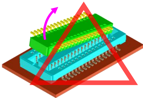
長手方向の斜め抜去 Slant releasing in "a" Direction (lengthways)
