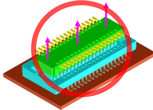
平行抜去 Releasing the plug paralleled to the mated axis
