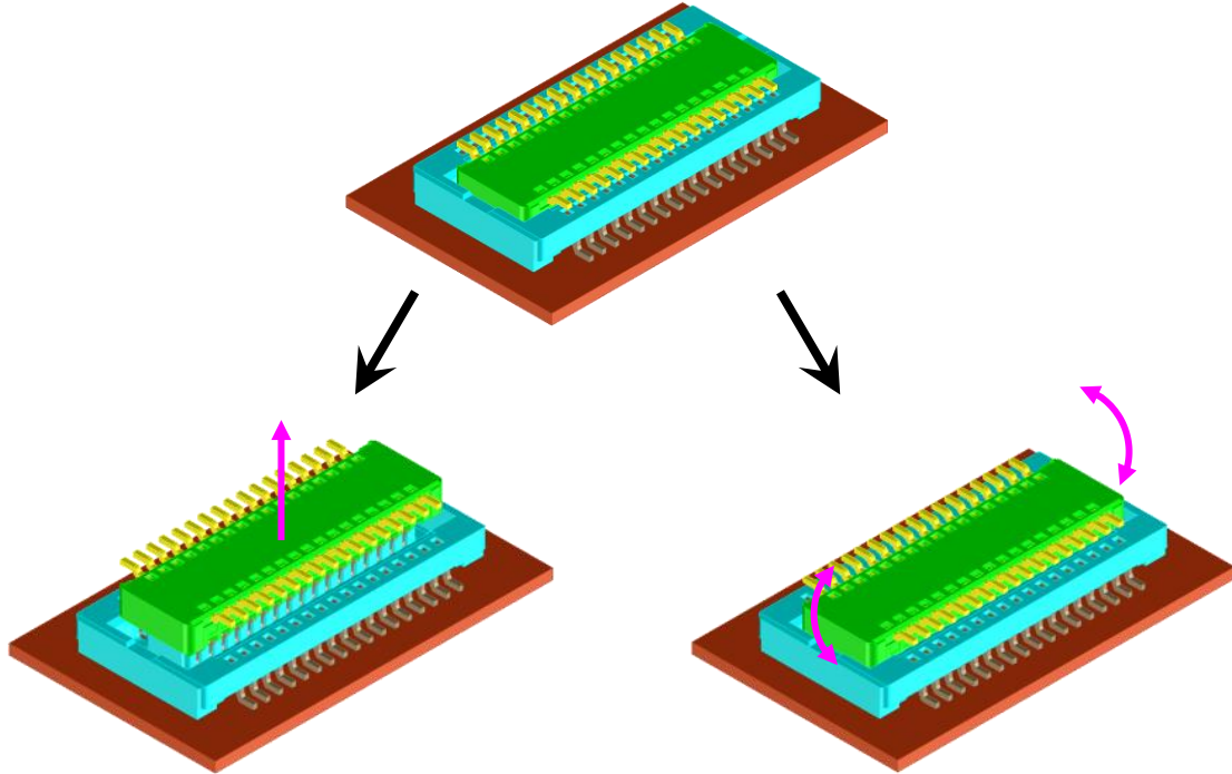
嵌合軸に沿って平行に抜く Releasing the plug paralleled to the mated axis
